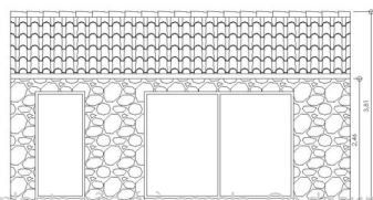
FACHADA PRINCIPAL
