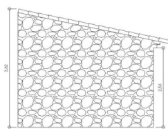
FACIENDA LATERAL I
