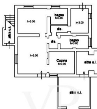
PIANO TERRA
