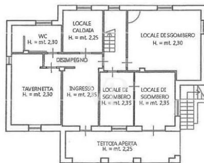
PIANO TERRA
