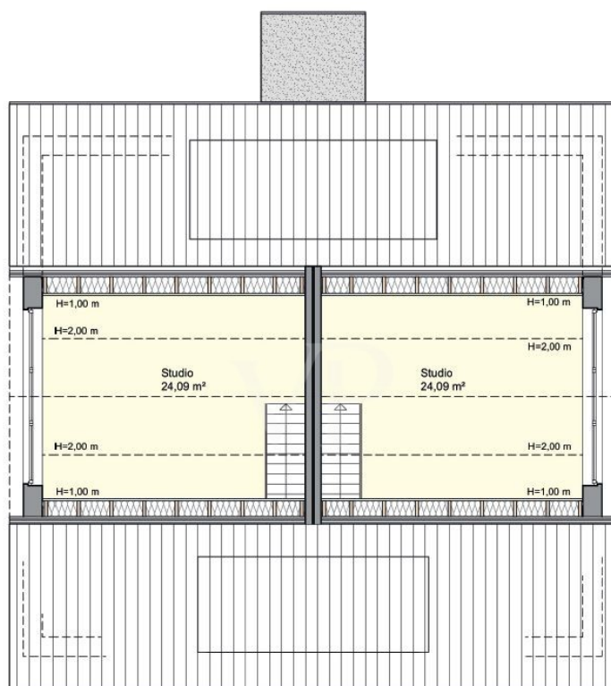
Grundriss Studio
